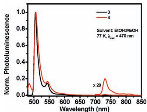
Figure 4. Normalized photoluminescence of 3 and 4 in a 77 K 4:1 EtOH/MeOH glass ( \lambda_{\text{ex}} = 470 nm). The phosphorescence of 4 ( \lambda_{\text{em}} = 733 nm) has been scaled by a factor of 20.
